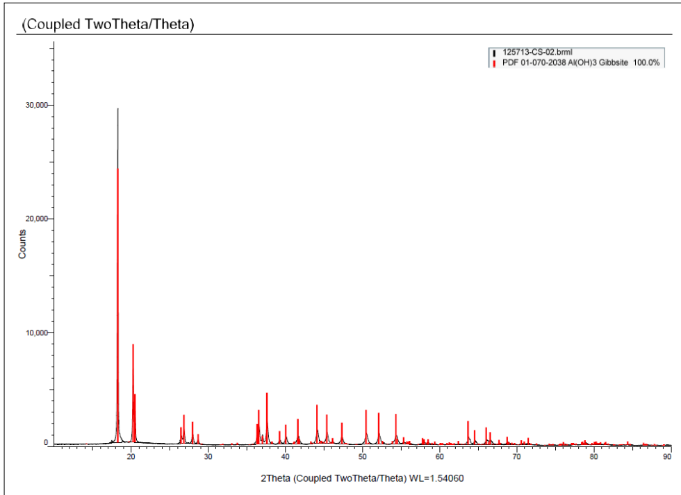
Fig2.1-1 “2312006236-2”XRD spectrogram
