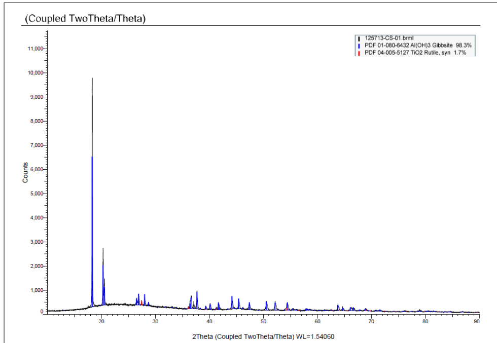
Fig2.1-1 “2312006236-1”XRD spectrogram
